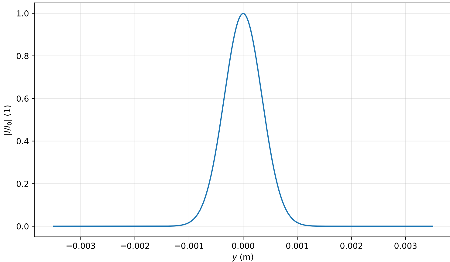
Intensity profile I(x=0, y, z=0.159)/I_0 , P_{in}=0.2P_{cr} , artificial time
